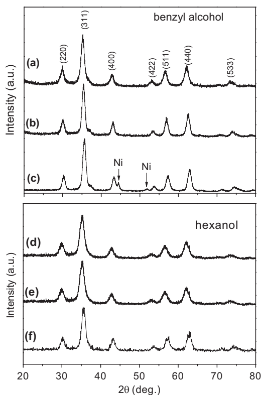
Fig. 1. XRD patterns of: (a) \text{MnFe}_2\text{O}_4 , (b) \text{CoFe}_2\text{O}_4 and (c) \text{NiFe}_2\text{O}_4 , synthesized in benzyl alcohol at 180^\circ\text{C}/24\text{h} ; (d) \text{MnFe}_2\text{O}_4 , (e) \text{CoFe}_2\text{O}_4 and (f) \text{NiFe}_2\text{O}_4 , synthesized in hexanol at 180^\circ\text{C}/24\text{h} .
