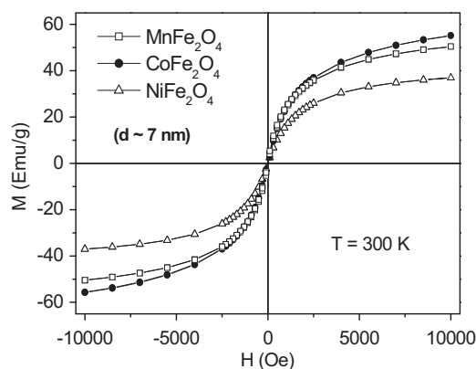
Fig. 6. Field-dependent magnetization measurements at RT of M\text{Fe}_2\text{O}_4 ( M = \text{Co}, \text{Ni}, \text{Mn} ) ferrites with particle diameter \sim 7 nm.
