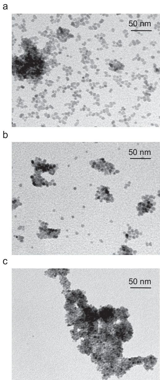
Fig. 3. TEM micrographs of \text{CoFe}_2\text{O}_4 prepared in benzyl alcohol at: (a) 180^\circ\text{C}/24\text{h} , (b) 190^\circ\text{C}/24\text{h} and (c) 180^\circ\text{C}/48\text{h} .
