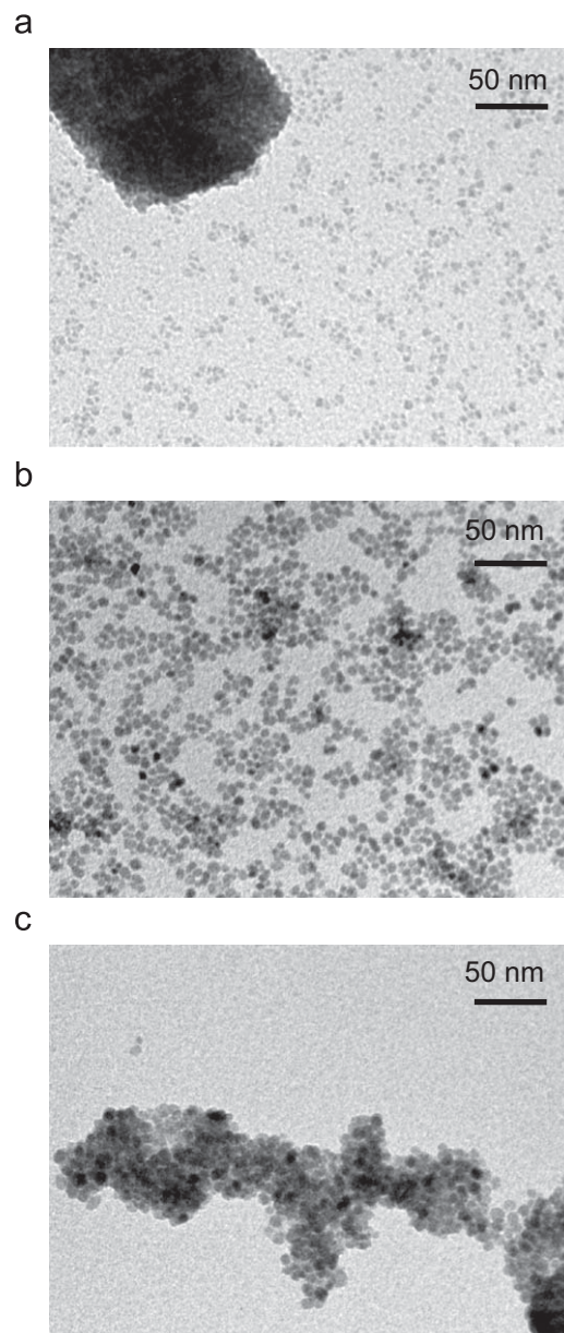
Fig. 2. TEM micrographs of: (a) \text{MnFe}_2\text{O}_4 , (b) \text{CoFe}_2\text{O}_4 and (c) \text{NiFe}_2\text{O}_4 synthesized in hexanol at 180^\circ\text{C}/24\text{h} .
