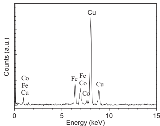
Fig. 5. EDS of \text{CoFe}_2\text{O}_4 particles prepared in benzyl alcohol at 180^\circ\text{C}/24\text{h} .
