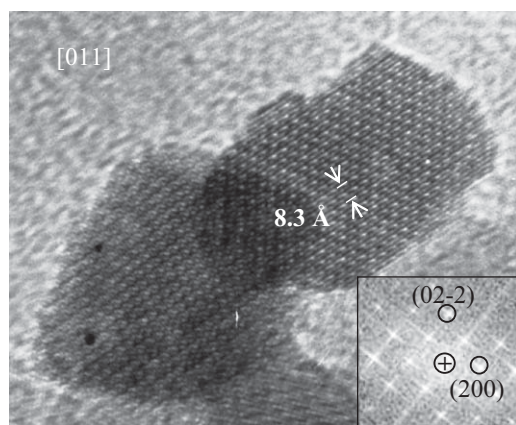
Fig. 4. High resolution transmission electron microscopy (HRTEM) image of \text{CoFe}_2\text{O}_4 prepared in benzyl alcohol at 180^\circ\text{C}/24\text{h} . Inset: the Fourier transform of the HREM image shows the electron diffraction pattern, which indicates that this particle is oriented along the zone axis [011].
